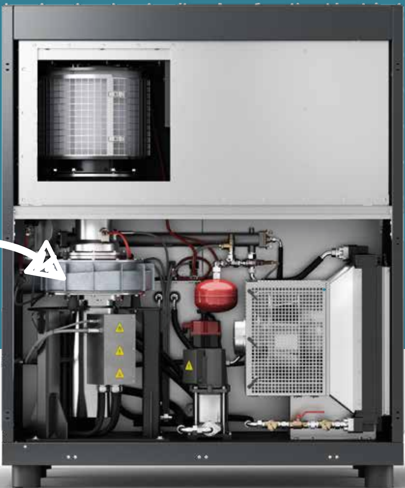
Image: Machine layout
